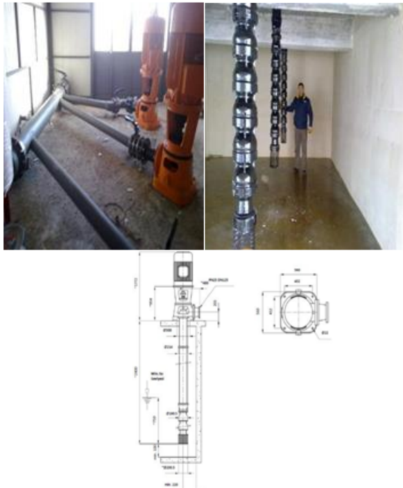
Figure 2. Parallel connected vertical pumps (Polat and Bowler, 2010)
